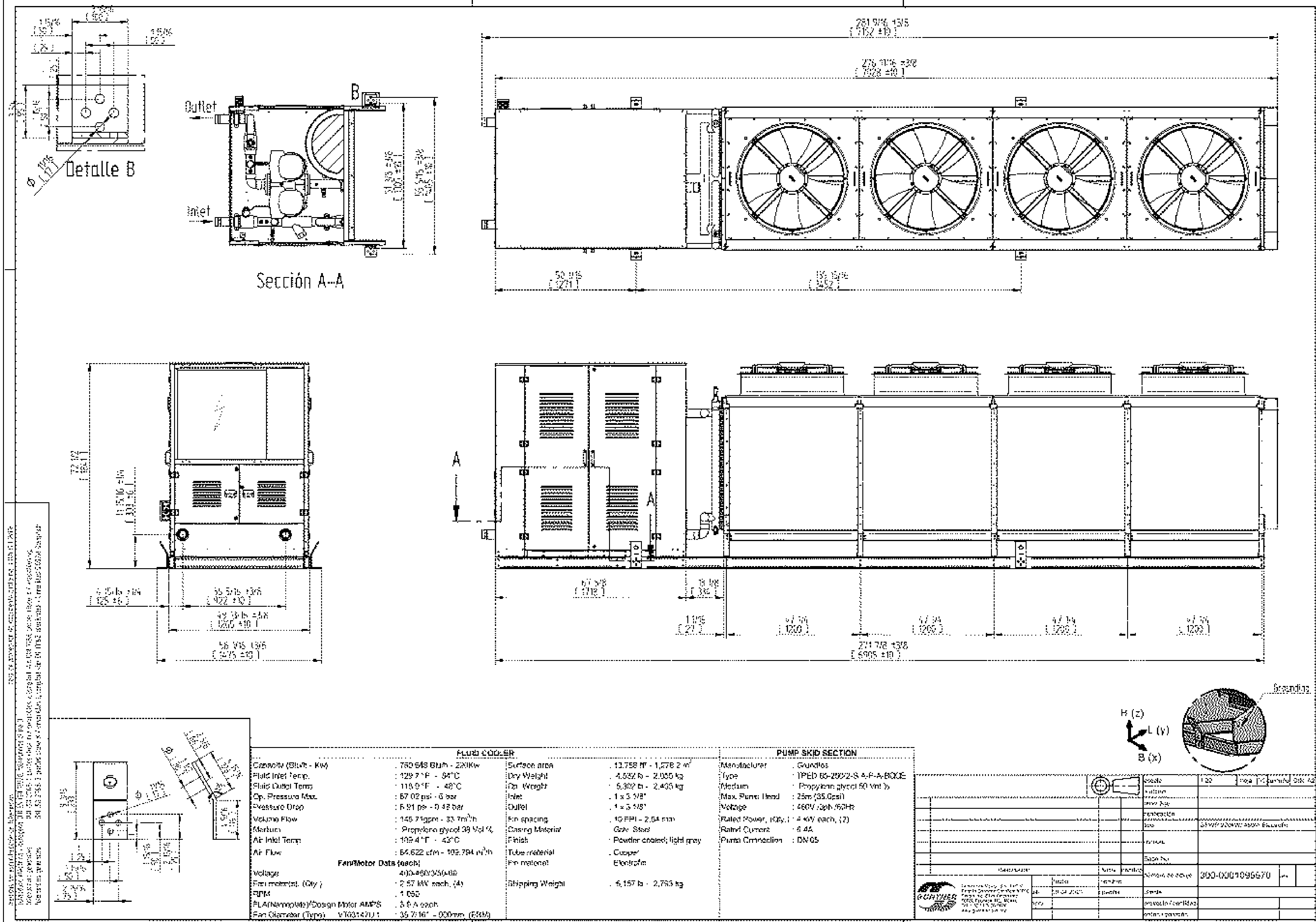
4-FAN DRY COOLER DETAIL
