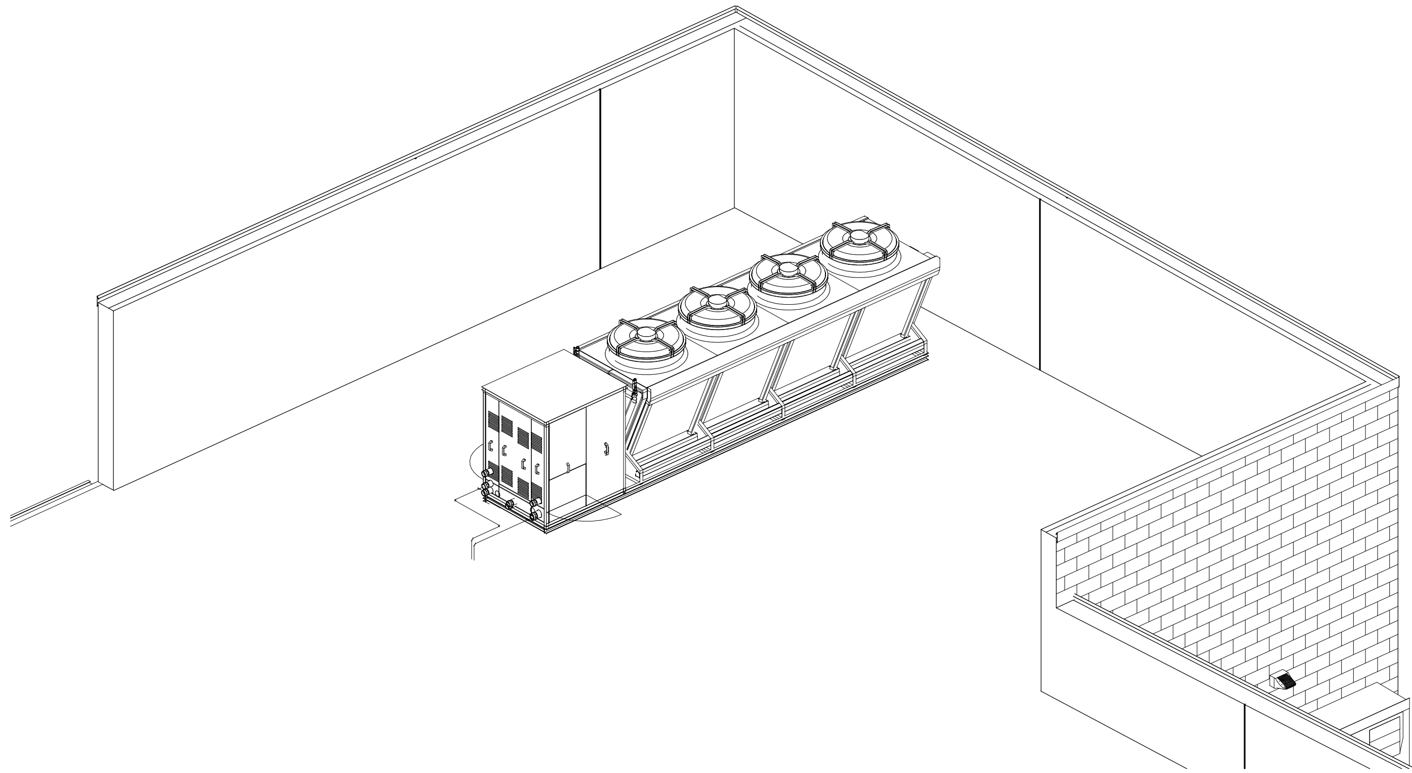
3 3D VIEW DRY COOLER #1
