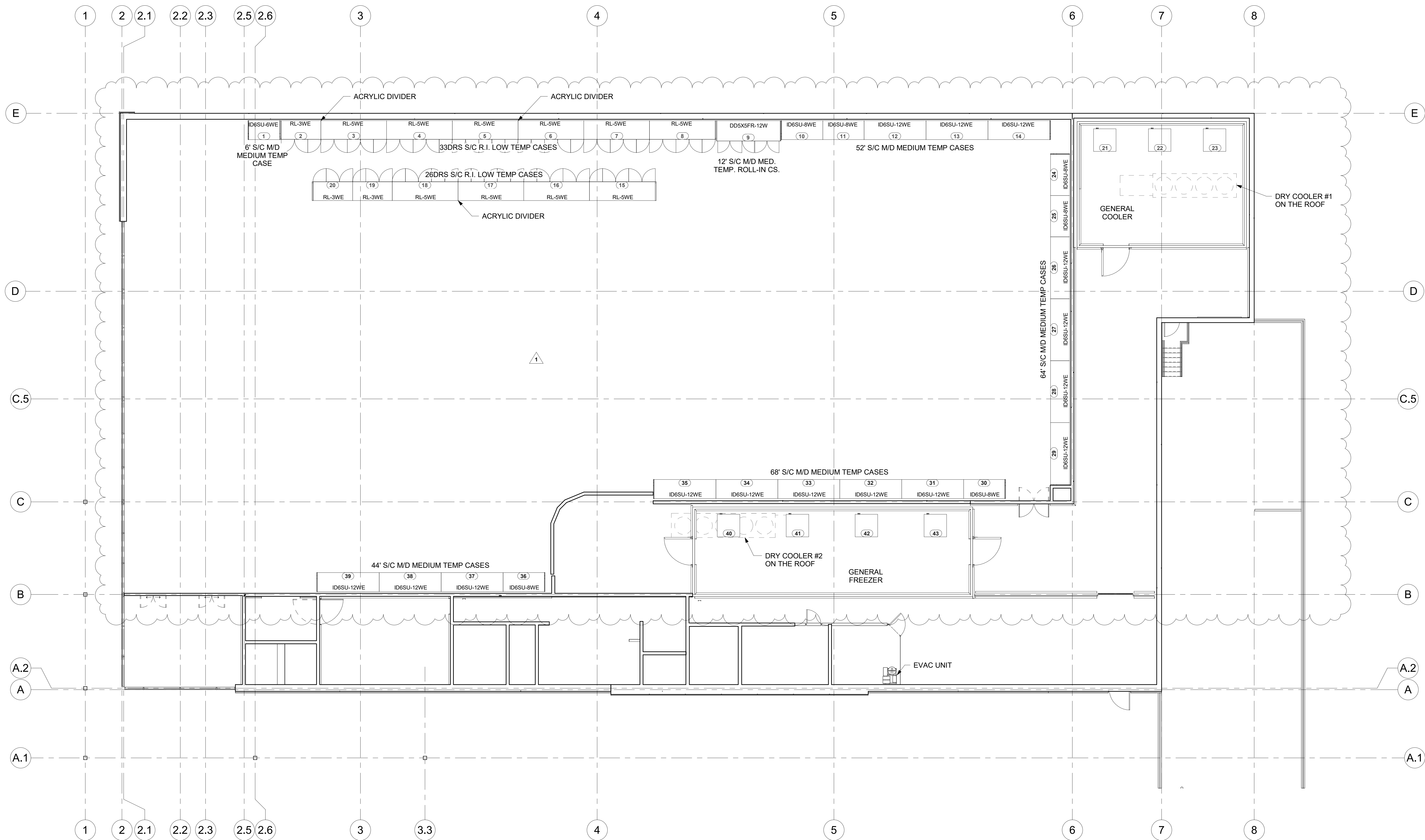
1 R1.0 FIXTURE FLOOR PLAN 1/8" = 1'-0"
