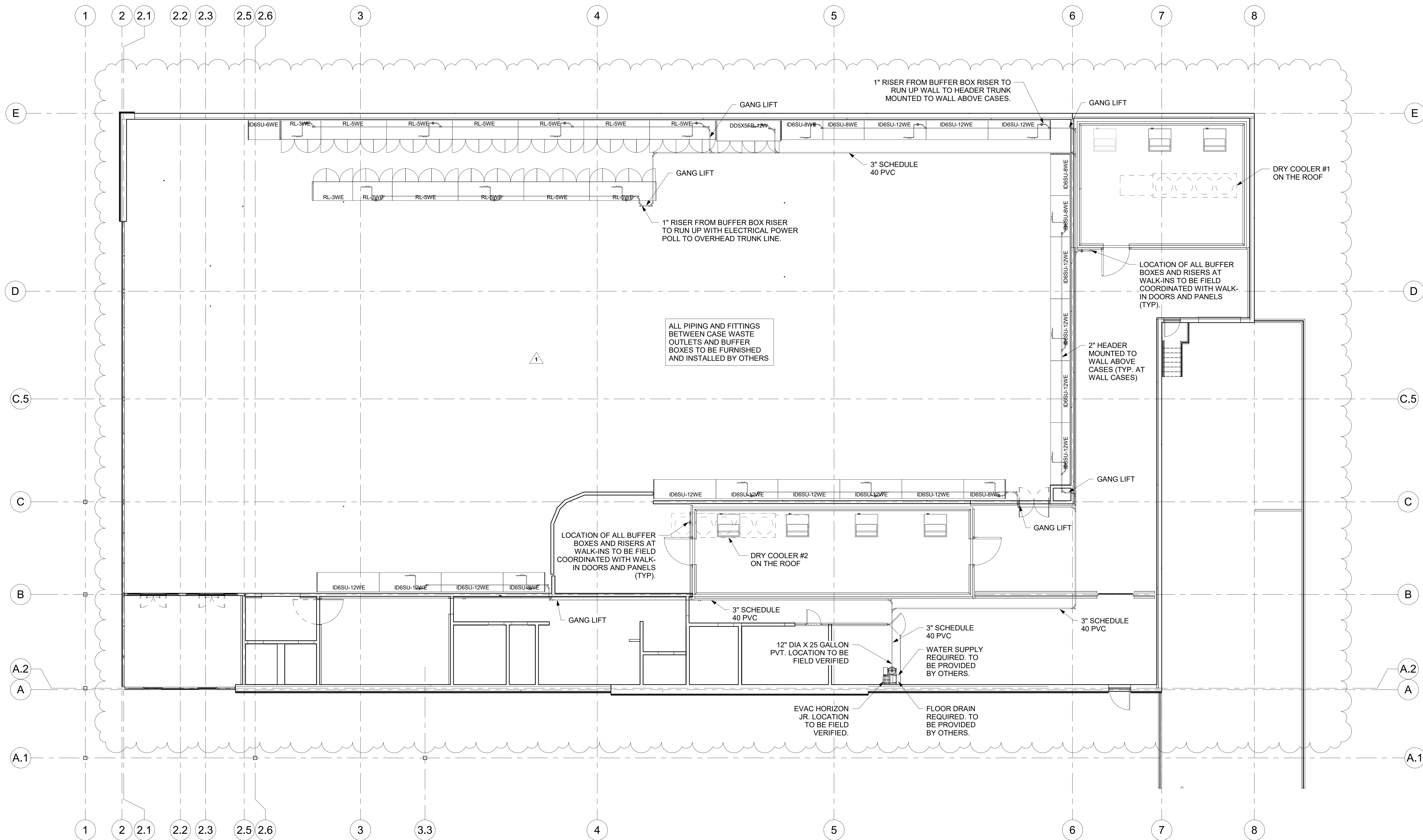
① R2.0 EVAC FLOOR PLAN 1/8" = 1'-0"
