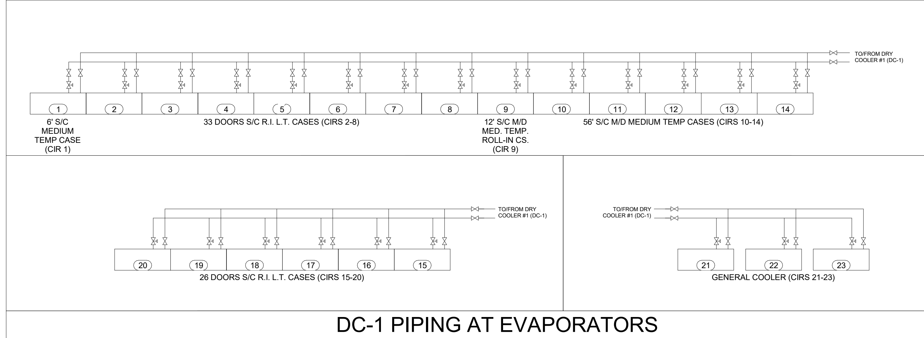
DC-1 PIPING AT EVAPORATORS
