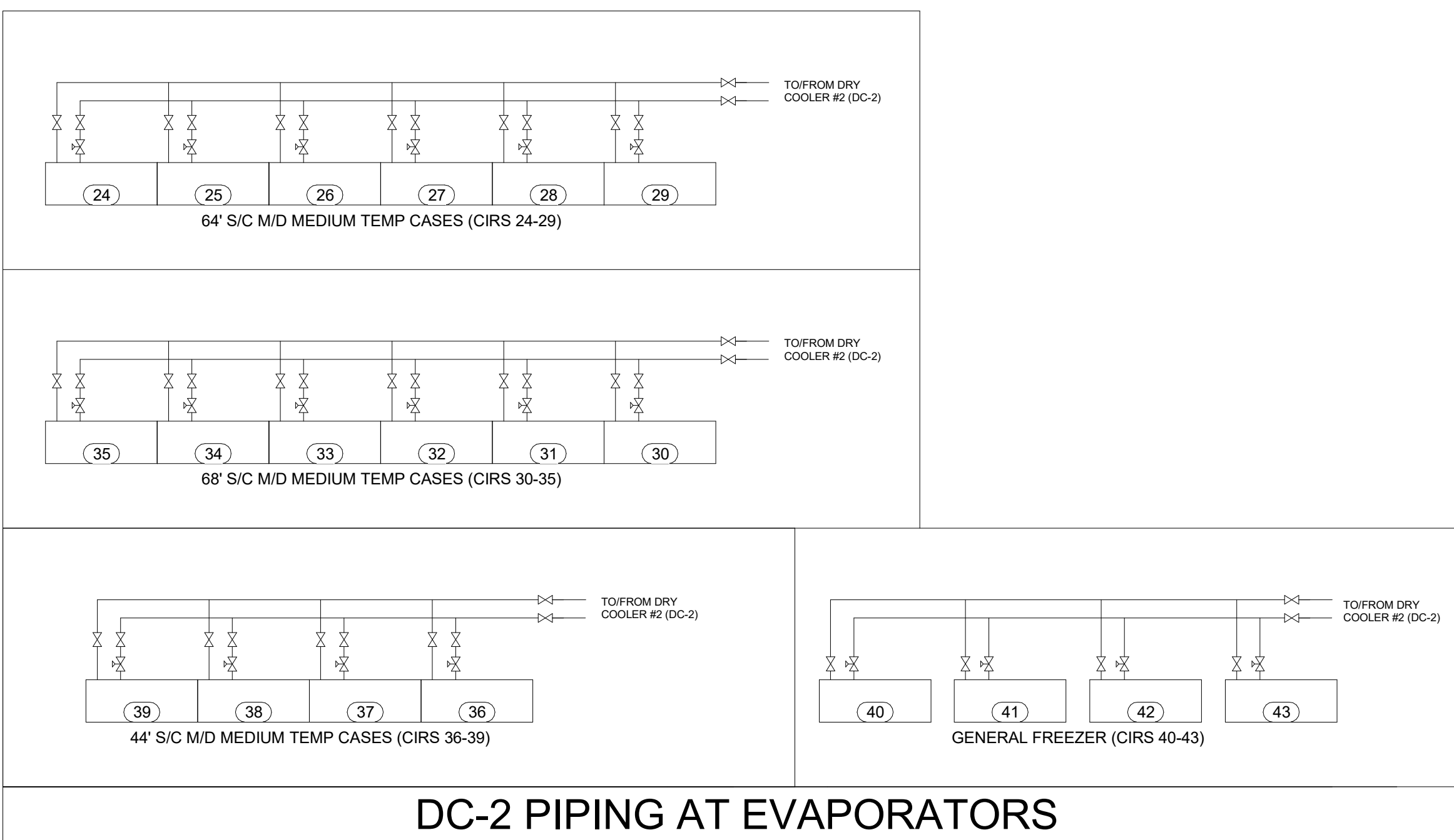
DC-2 PIPING AT EVAPORATORS
