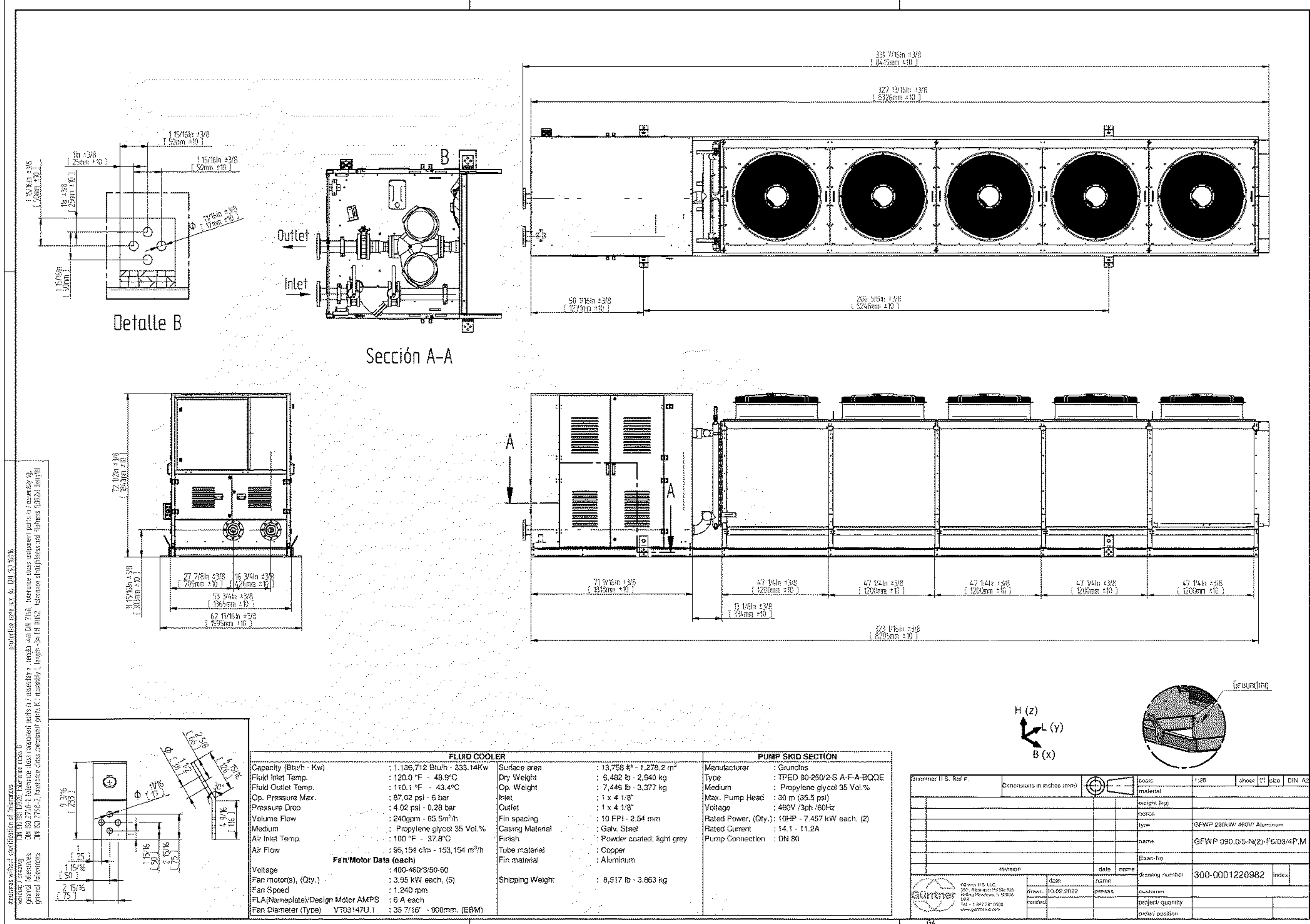
5-FAN DRY COOLER DETAIL
